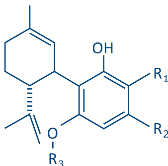
FIGURE 2. Cannabinoids of the CBD type. The most widespread cannabinoids are the phenolic CBD ( R_1 = H ) with 21 carbon atoms and a C5 side chain ( R_2 = C_5H_{11} ) and its corresponding carboxylic acid ( R_1 = COOH ).
