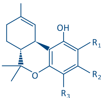
FIGURE 1. Cannabinoids of the THC type. The most widespread cannabinoids are the \Delta^9 THC with 21 carbon atoms and a C5 side chain ( R_2 = C_5H_{11} ) and its two corresponding carboxylic acids A and B.
